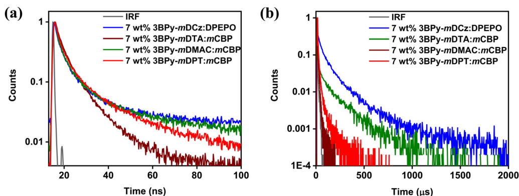
Fig. 4 Transient PL decays of DPEO and mCBP host films doped with 7 wt% of emitter (a) prompt and (b) delayed component at 298 K.
