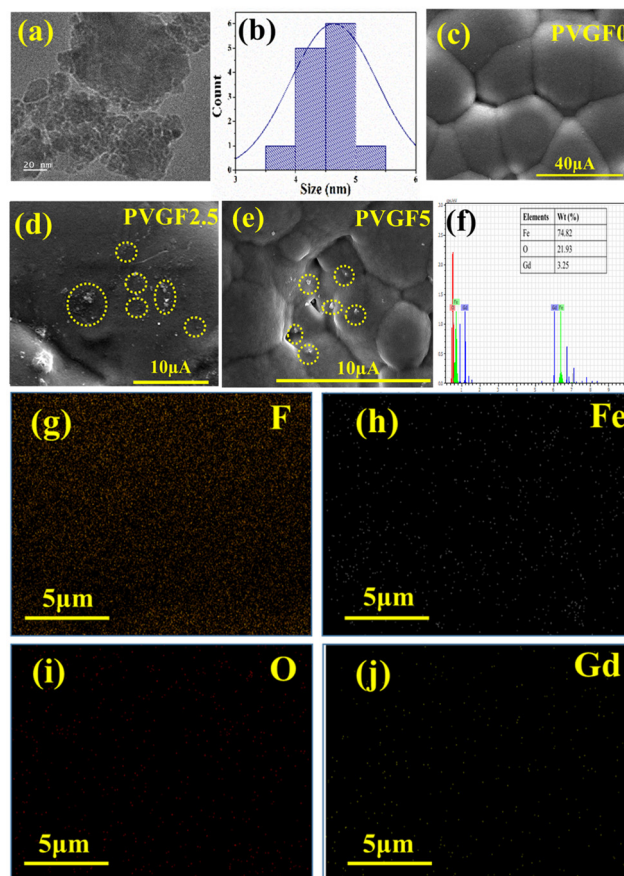
Fig. 2 (a) and (b) TEM image and the size distribution curve of Gd-incorporated \alpha -hematite. (c)–(e) FESEM micrographs of PVGF0, PVGF2.5, PVGF5. (f) EDX image Gd-incorporated hematite NPs. (g)–(j) Mapping of the PVGF2.5 membrane suggesting the homogeneous distribution of doped-Gd-incorporated hematite in the PVDF matrix. The carbon distribution of the membrane is not shown due to the use of carbon tape during the EDS mapping measurement.
