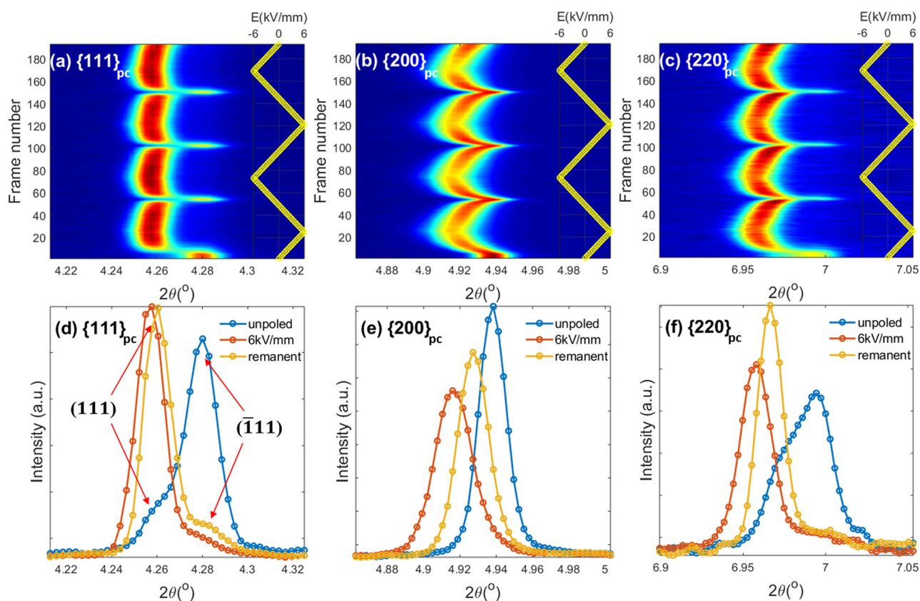
Fig. 7 Contour plots of Nb-doped 0.7BF-0.3BT ceramics at 125 °C of the \{111\}_{pc} , \{200\}_{pc} and \{220\}_{pc} reflections under 2 bipolar electric field cycles in (a), (b) and (c) respectively, and comparison of peak profiles for the unpoled state, under 6 kV mm -1 and in the remanent state in (d), (e) and (f).
