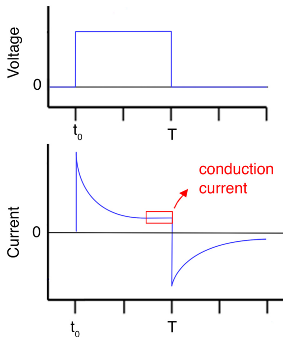
Fig. 11 Double-pulsed, controlled potential chronoamperometry. A square wave voltage initially causes a current peak, due to polarisation. The current then exponentially decays to the conduction current. The removal of the voltage may cause a brief reversed current peak.
