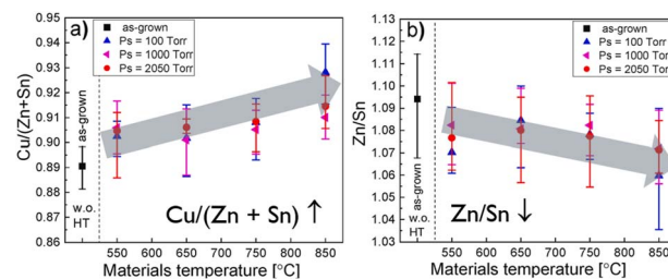
Fig. 4 (a) \text{Cu}/(\text{Zn} + \text{Sn}) and (b) \text{Zn}/\text{Sn} compositional ratios of the CZTS MGP crystals depending on the post-annealing regime as determined by EDX. Reproduced from ref. 34 with permission from Elsevier B.V., Copyright 2022.
