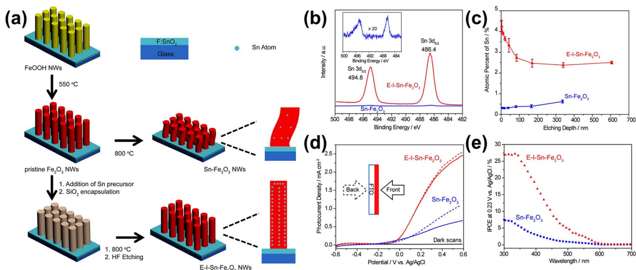
Fig. 9 (a) Schematic illustration of the preparation of \text{Sn-Fe}_2\text{O}_3 NWs and E-I-Sn- \text{Fe}_2\text{O}_3 NWs. (b) XPS Sn 3d spectra of \text{Sn-Fe}_2\text{O}_3 and E-I-Sn- \text{Fe}_2\text{O}_3 . Inset: magnified Sn 3d spectrum of \text{Sn-Fe}_2\text{O}_3 . (c) SIMS depth profiles of \text{Sn-Fe}_2\text{O}_3 and E-I-Sn- \text{Fe}_2\text{O}_3 . Error bars are evaluated based on parallel experiments. (d) J-V curves of \text{Sn-Fe}_2\text{O}_3 and E-I-Sn- \text{Fe}_2\text{O}_3 collected at 20 \text{mV s}^{-1} in a 1.0 M KOH aqueous electrolyte under one sun illumination ( 100 \text{ mW cm}^{-2} ) and in the dark. The solid and dashed lines represent the data collected under the front (solid lines) and back (dashed lines) illuminations, respectively. (e) IPCE spectra of \text{Sn-Fe}_2\text{O}_3 and E-I-Sn- \text{Fe}_2\text{O}_3 collected at 0.23 V vs. Ag/AgCl. Reproduced from ref. 63 with permission from American Chemical Society, Copyright 2017.
