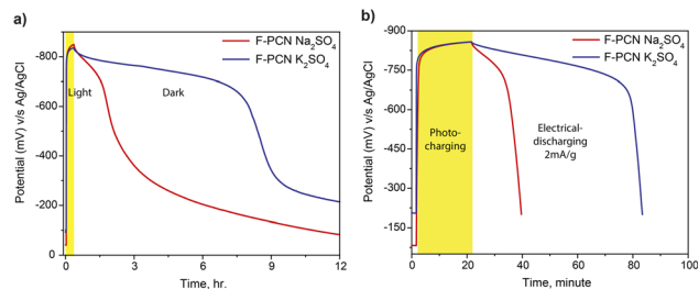
Fig. 4 (a) OCP measurement on F-PCN in the presence of different electrolytes ( \text{M}_2\text{SO}_4 and 4-MBA) (b) Photo charging of F-PCN in the presence of different electrolytes for 20 minute (OCP) and subsequently electrical discharging with 2 \text{ mA g}^{-1} . All the measurements are done in an inert condition.
