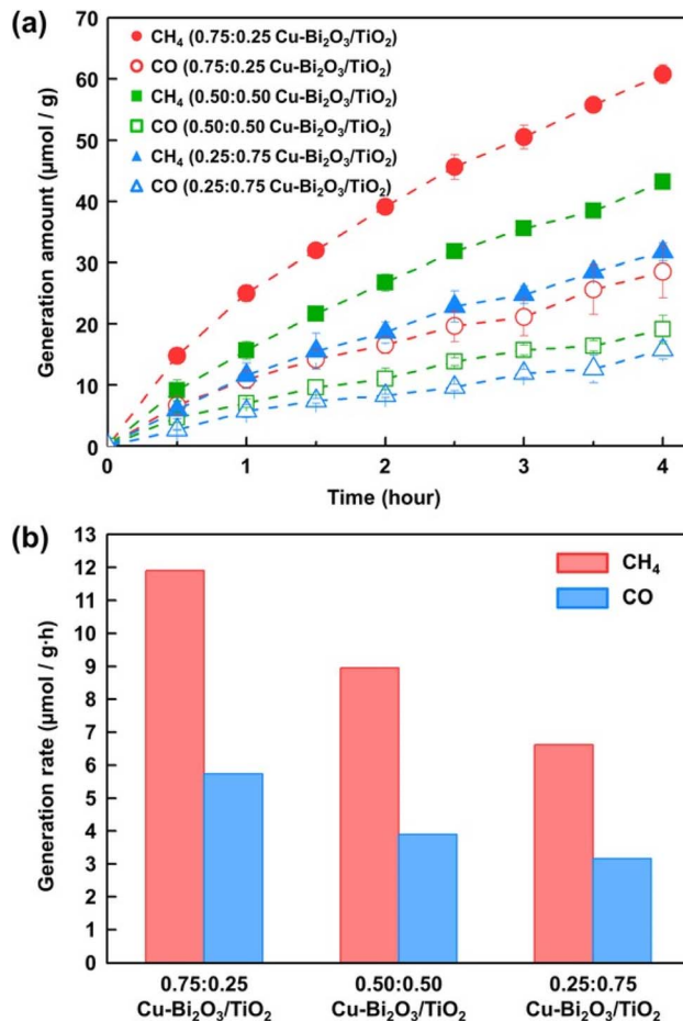
Fig. 18 (a) Amount of \text{CH}_4 and \text{CO} generated upon using 0.75 : 0.25, 0.50 : 0.50, and 0.25 : 0.75 \text{Cu-Bi}_2\text{O}_3/\text{TiO}_2 photocatalysts. (b) Rates of \text{CH}_4 and \text{CO} generation in the first 4 h of irradiation. Reproduced with permission from ref. 217, Copyright 2016 European Chemical Societies Publishing.
