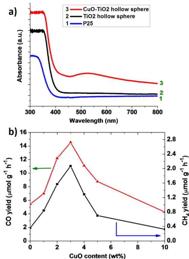
Fig. 17 (a) UV-vis DRS for various \text{TiO}_2 based nano-materials. The CuO content in the \text{CuO-TiO}_2 catalyst is 3 wt%. (b) Yields of the gas products ( \text{CO} and \text{CH}_4 ) produced during 24 h of photo-driven \text{CO}_2 reduction on the \text{TiO}_2 hollow microsphere catalysts with various Cu contents. Reproduced with permission from ref. 194, Copyright 2015 American Chemical Society.
