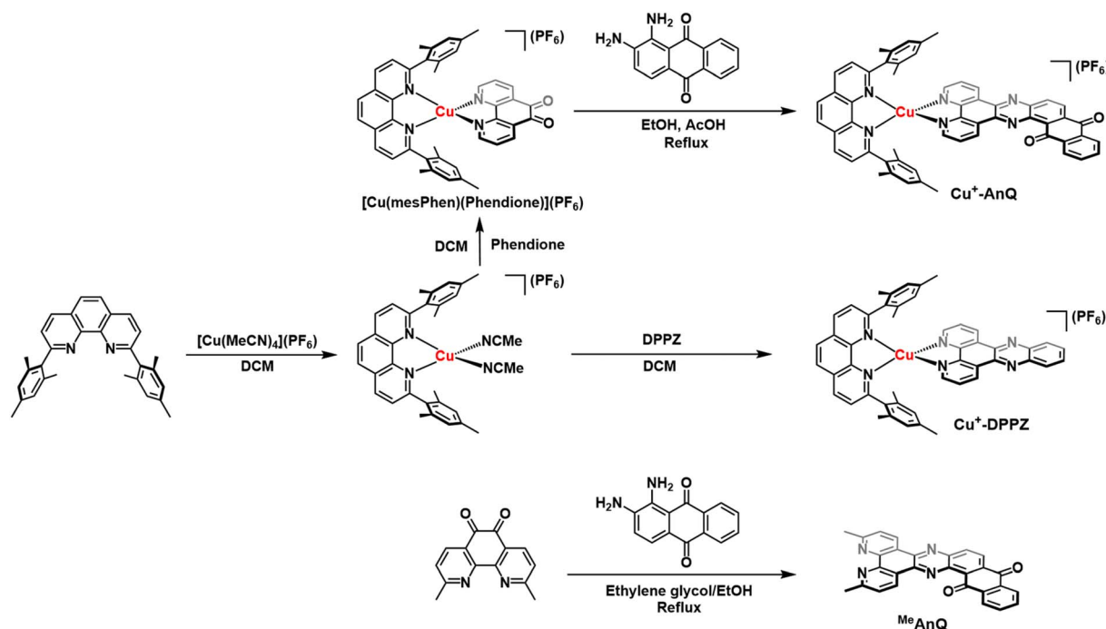
Scheme 1 Synthesis of Cu + -AnQ , Cu + -DPPZ and Me AnQ .
