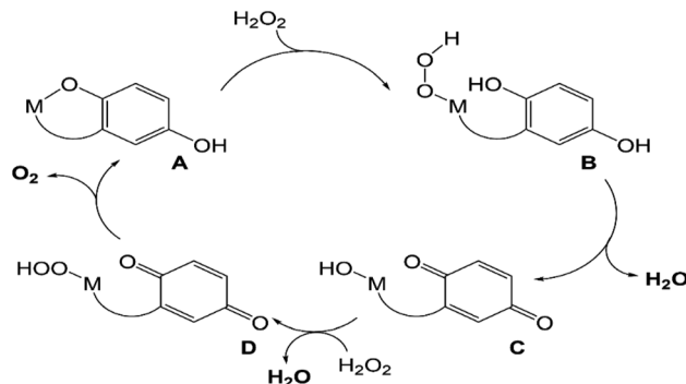
Scheme 4 Proposed mechanism for catalase activity that avoids metal-centered redox.
