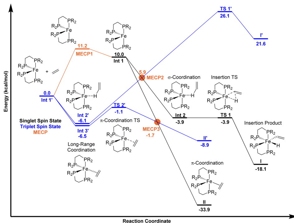
Fig. 2 M06-L potential energy landscapes for reaction between (DMPE) 2 Fe and ethylene. Black numbers and lines represent unrestricted singlet spin-state energies. Blue numbers and lines represent unrestricted triplet spin-state energies. Orange dots give MECP energies. Energies are reported in kcal mol -1 (R = Me).
