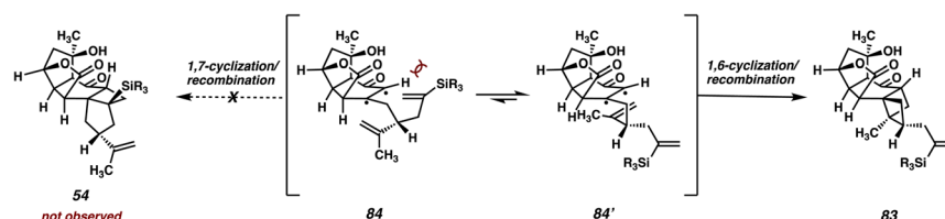
Fig. 5 Mechanistic rationale for the undesired photocycloaddition outcome.
