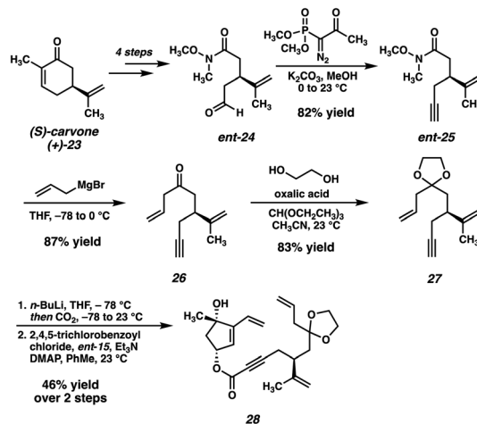
Scheme 3 Synthesis of RCM substrate 28 .
