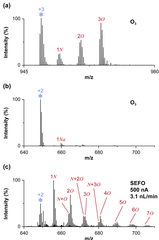
Fig. 7 Oxidation by ozone. (a) Oxidation of 10 \mu M melittin in 100 mM ammonium formate using ozone produced from the DBD source. (b) Oxidation of 20 \mu M angiotensin I in 50 mM HCl using ozone. (c) Strong electric field-induced oxidation of angiotensin I in 500 mM HCl. Asterisk denotes the unoxidized peak.
