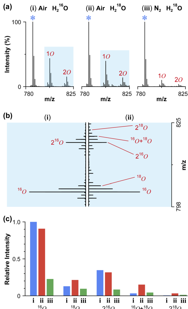
Fig. 8 Measurement using the oxygen isotope. (a) Mass spectra obtained under oxidized conditions for 5 \mu M L-phosphatidylcholine (PC 18 : 1/18 : 1) in 500 mM HCl prepared using normal water (i) and water- ^{18}O (ii & iii). The operating gases are air (i & ii) and high-purity nitrogen (iii). Asterisk denotes the peak without oxidation. (b) Enlarged view of (a) (i) and (a) (ii). (c) Intensity comparison for different oxidation species.
