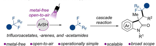
Fig. 1 Previous approaches to preparing difluoroalkylated compounds.
