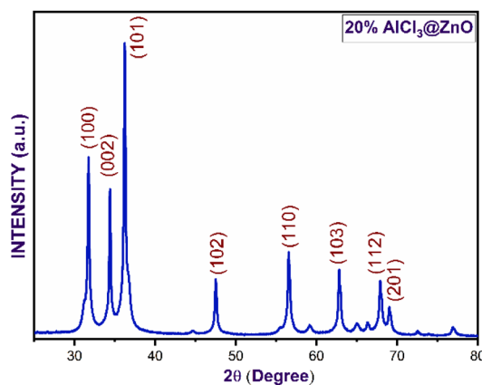
Fig. 12 XRD of recovered 20% \text{AlCl}_3\text{@ZnO} nanocatalyst after 4 h of drying at 120 °C.
