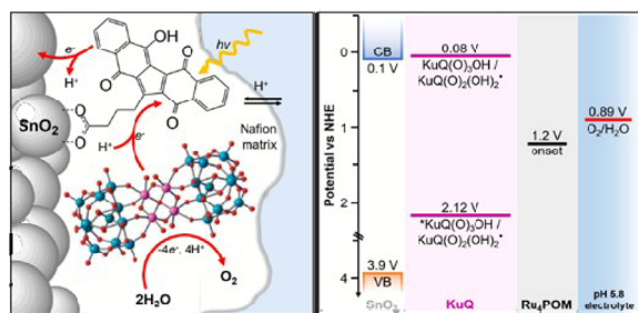
Fig. 11 Schematic representation of Ru 4 POM|KuQ3CO 2 H|SnO 2 photoanodes for water oxidation. The energy levels are shown for the system at pH = 5.8. Reproduced from ref. 72 with permission from the Royal Society of Chemistry.
