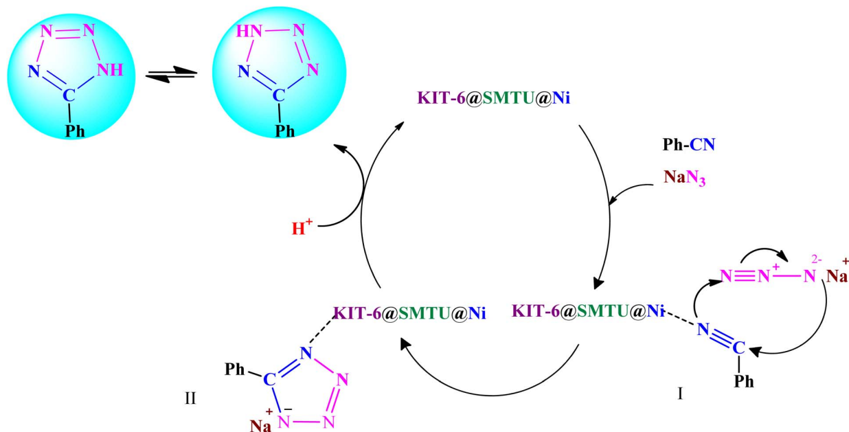
Scheme 4 The proposed mechanism for the synthesis of tetrazoles in the existence of \text{KIT-6@SMTU@Ni} .
