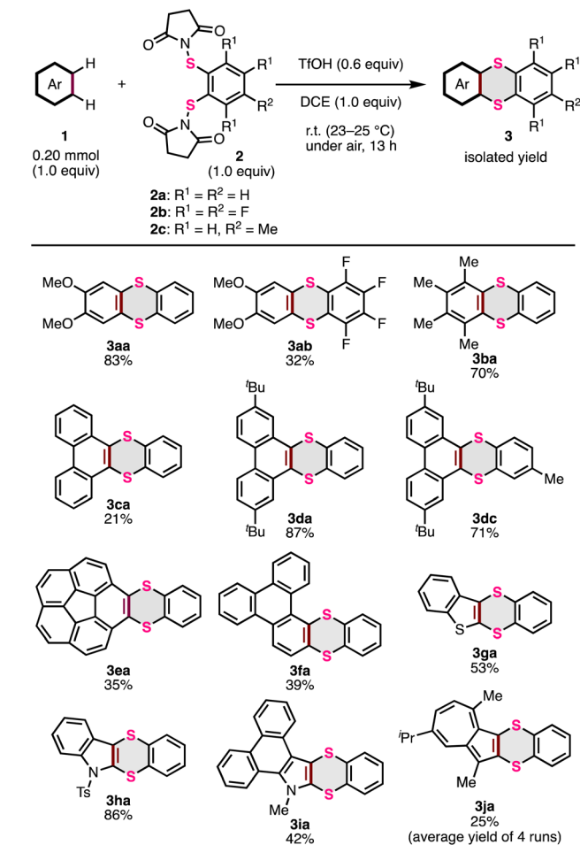
Fig. 3 Scope of substrates in the thia-APEX reaction.
