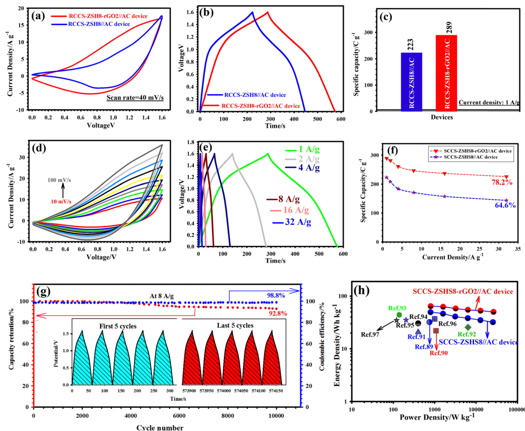
Fig. 10 (a) CV curves of the RCCS-ZSH8-rGO2//AC devices at 40 mV s -1 . (b) GCD curves of the RCCS-ZSH8//AC and RCCS-ZSH8-rGO2//AC devices at 1 A g -1 . (c) Specific capacities of RCCS-ZSH8//AC and RCCS-ZSH8-rGO2//AC devices at 1 A g -1 . (d) CV plots of the RCCS-ZSH8-rGO2//AC at various sweep speeds of 10–100 mV s -1 . (e) GCD plots of the RCCS-ZSH8-rGO2//AC at various current densities of 1–32 A g -1 . (f) Specific capacity vs. current density of the RCCS-ZSH8//AC and RCCS-ZSH8-rGO2//AC devices. (g) Durability and coulombic efficiency of the RCCS-ZSH8-rGO2//AC at 8 A g -1 (the inset shows the first and last 5 GCD cycles). (h) The comparison of the RCCS-ZSH8-rGO2//AC device's Ragone plot with those of various devices.
