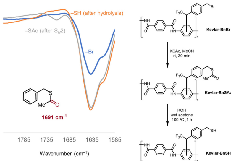
Fig. 3 IR transmission spectrum of Kevlar sample after benzyl–bromide diazire attachment (blue), thioacetate treatment (grey), and base hydrolysis of the thioester group (orange).
