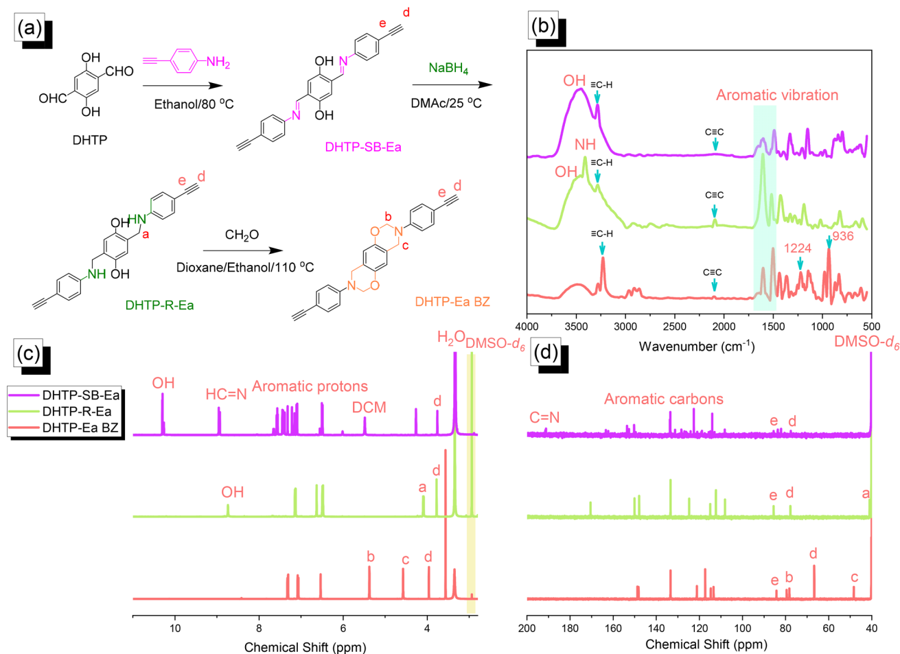
Fig. 2 (a) Synthesis of DHTP-Ea BZ from DHTP, DHTP-SB-Ea, and DHTP-R-Ea. (b-d) Corresponding (b) FTIR, (c) 1 H NMR, and (d) 13 C NMR spectra.
