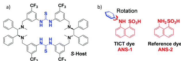
Fig. 12 Chemical structures of the chiral host (a), and the achiral fluorescent guest (b). Adopted with permission from ref. 142. Copyright 2020, Royal Society of Chemistry.
