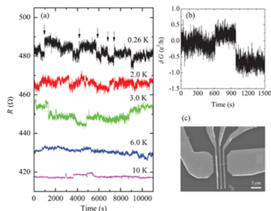
Fig. 16 (a) Resistance at five temperatures for a RuO 2 NW with length L = 1.5 μm and diameter d = 67 nm. Data at 6.0 K, 3.0 K, 2.0 K, and 0.26 K are offset by 10 Ω, 20 Ω, 30 Ω, and 40 Ω, respectively, for clarity. (b) Conductance variation \delta G = G - \langle G \rangle vs. time at 0.26 K. (c) Scanning electron microscope (SEM) image of lithographically defined NW. Reproduced from ref. 65 with permission. Copyright 2011 American Institute of Physics.
