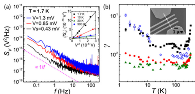
Fig. 17 (a) S_V vs. f and T for an IrO 2 NW with L = 0.9 μm and d = 147 nm; \langle S_V \rangle vs. V^2 is shown in the inset. (b) \gamma = S_V N_c f / V^2 vs. T for IrO 2 NWs from 1.7 K to 350 K. The inset is a SEM image of a NW. Dimensions are L = 1.9 μm, d = 143 nm (solid black squares); L = 1.0 μm, d = 123 nm (solid red circles); L = 0.75 μm, d = 125 nm (solid green triangles); and L = 0.9 μm, d = 147 nm (open blue diamonds). Reproduced from ref. 75 with permission. Copyright 2023 American Institute of Physics.
