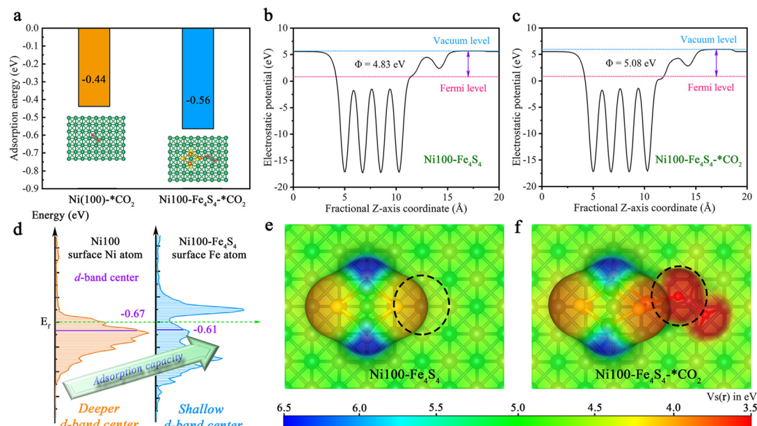
Fig. 4 The adsorption energy, d-band center, surface electrostatic potential and work function analysis of CO 2 adsorption. (a) Comparison of the adsorption energies between Ni (100) and Ni100–Fe 4 S 4 . (b) The work function of Ni100–Fe 4 S 4 . (c) The work function of Ni100–Fe 4 S 4 *CO 2 . (d) Comparison of the d-band centers between the Ni atom on Ni (100) and the Fe atom on Ni100–Fe 4 S 4 . (e) Electron-density isosurface of Ni100–Fe 4 S 4 . (f) Electron-density isosurface of Ni100–Fe 4 S 4 *CO 2 . The color bar stands for the scale of the electrostatic potential and the isosurfaces are plotted at the 0.002 e bohr −3 level.
