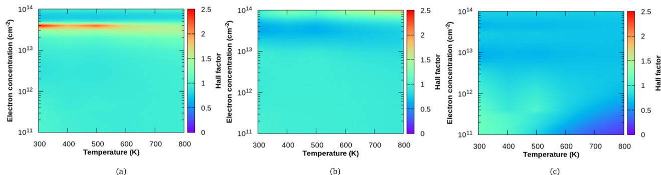
Fig. 5 Variation of the Hall factor in terms of temperature and concentration for (a) \text{Sc}_2\text{CF}_2 , (b) \text{Sc}_2\text{CO}_2 and (c) \text{Sc}_2\text{C}(\text{OH})_2 .
