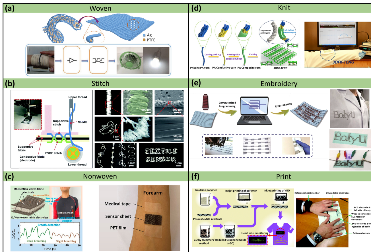
Fig. 5 Yarn/fabric-based breathable skin-mountable electronics. (a) Schematic diagram of a co-axially structured adaptive textile and a textile in a smart home control system. Reproduced with permission from ref. 102. Copyright 2019 Wiley-VCH. (b) Schematic diagram of a textile sensor manufactured using a sewing machine and a photograph, SEM images of a PVDF stripe stitch. SEM image of the interface between AgNWs and PU NFs. Reproduced with permission from ref. 103. Copyright 2018 Royal Society of Chemistry. (c) Schematic diagram of the preparation of a fabric pressure sensor, which was successfully sewn into a tight-fitting, quick-drying garment and used to measure the respiration rate of the wearer. Schematic diagram of PET film, medical tape, and breathable sensor covering the front of the skin. Reproduced with permission from ref. 104. Copyright 2022 American Chemical Society. (d) The fabrication process of the core-sheath yarn and TENG. Reproduced with permission from ref. 105. Copyright 2020 Elsevier. (e) Schematic diagram of the preparation of conductive silver-plated nylon yarn. Reproduced with permission from ref. 106. Copyright 2019 SpringerLink. (f) Schematic diagram of the entire inkjet-printed graphene textile manufacturing process and experimental image of two fingers placed on a printed graphene patch. Reproduced with permission from ref. 107. Copyright 2017 Royal Society of Chemistry.
