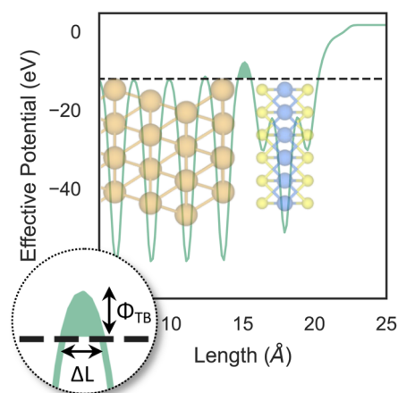
Fig. 6 Effective potential across the interface of the pristine Au/ \text{MoS}_2 structure. The potential was projected in the direction of the interface. Highlighted in the figure are the tunnelling barrier height ( \Phi_{\text{TB}} ) and the barrier width ( \Delta L ).
