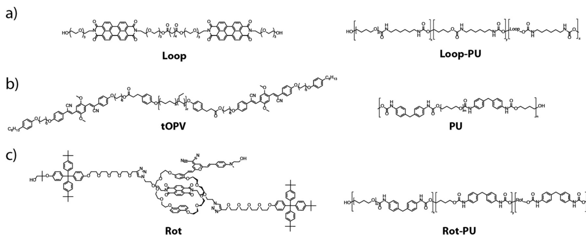
Fig. 1 Chemical structures of the three mechanophores investigated in this work, as well as the polymers into which they were incorporated. (a) Loop-forming perylenediimide-based mechanophore ( Loop ) and the Loop -containing polyurethane ( Loop-PU ) based on hexamethylene diisocyanate, butane diol (BDO), and poly(tetrahydrofuran) (poly(THF)). (b) Telechelic cyano-OPV-functionalised poly(ethylene-co-butylene) ( tOPV ) and a polyurethane ( PU ) based on methylene diphenyl diisocyanate (MDI), BDO, and poly(THF). (c) Rotaxane-based mechanophore ( Rot ) and the Rot -containing polyurethane ( Rot-PU ) based on MDI, BDO, and poly(THF).
