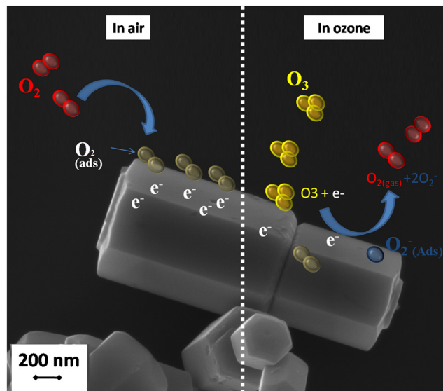
Fig. 7 FESEM image of ZnO nanorods synthesized via a hydrothermal method and the schematic ozone sensing mechanism.
