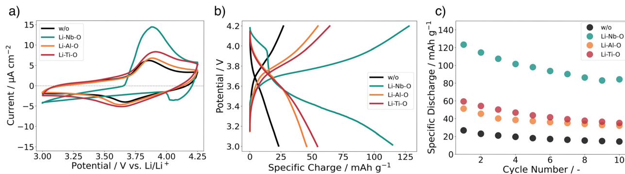
Fig. 6 (a) Cyclic voltammetry scans measured with a sampling rate of 0.1 \text{ mV s}^{-1} between 3 and 4.25 \text{ V vs. Li/Li}^+ , (b) charge–discharge curves with 1.75 \mu\text{A cm}^{-2} between 3 V and 4.2 V at 80^\circ\text{C} , and (c) specific discharge capacities for full cells with and without interface modification.
