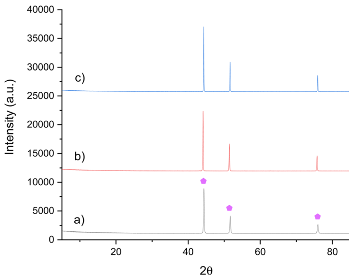
Fig. 11 XRD patterns of \text{Ni}_3\text{Cu} : (a) pre \text{N}_2 treatment, (b) post \text{N}_2 treatment at 700 °C and (c) post \text{N}_2 treatment at 800 °C. \blacklozenge \text{Ni}_3\text{Cu} .
