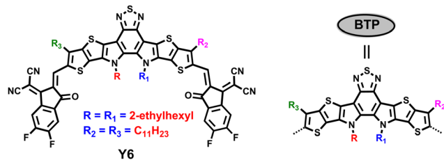
Fig. 13 The chemical structures of Y6 and BTP.
