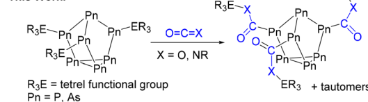
Fig. 1 Previously reported reactions of [\text{Pn}_7] clusters with small molecules and this work.
