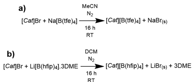
Scheme 1 Generalised reaction schemes for the metathesis of the (a) [\text{B}(\text{tfe})_4]^- and (b) [\text{B}(\text{hfp})_4]^- ILs where [\text{Cat}]^+ represents either [\text{N}_2(2\text{O}_2\text{O}_1)_3]^+ , [\text{P}_{12214}]^+ or [\text{C}_3\text{mpyr}]^+ . Note: for [\text{P}_{12214}]^+ , the tosylate ( [\text{H}_3\text{C}(\text{C}_6\text{H}_4)\text{SO}_3]^- ) salt is used instead of \text{Br}^- . MeCN is acetonitrile and DCM is dichloromethane.
