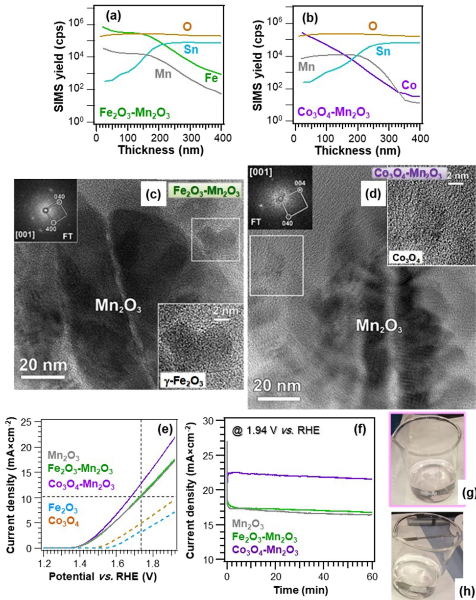
Fig. 5 Secondary ion mass spectrometry (SIMS) depth profiles of \text{Fe}_2\text{O}_3 - \text{Mn}_2\text{O}_3 (a) and \text{Co}_3\text{O}_4 - \text{Mn}_2\text{O}_3 deposits (b) obtained by plasma enhanced-chemical vapor deposition (PE-CVD) of manganese oxides on FTO, functionalization with \text{Fe}_2\text{O}_3 and \text{Co}_3\text{O}_4 by sputtering, and final annealing under an Ar atmosphere. (c) HR-TEM image of an \text{Fe}_2\text{O}_3 - \text{Mn}_2\text{O}_3 specimen. The white box marks a single \text{Fe}_2\text{O}_3 particle, whose enlargement is given as an inset. The corresponding Fourier transform (FT) pattern ([001] zone axis) in the upper left corner highlights the occurrence of cubic \gamma - \text{Fe}_2\text{O}_3 polymorph. (d) HR-TEM image of a \text{Co}_3\text{O}_4 - \text{Mn}_2\text{O}_3 sample. The white box marks a single \text{Co}_3\text{O}_4 nanoparticle, whose enlargement is provided as an inset. The corresponding FT pattern ([001] zone axis) in the top left corner indicates the presence of cubic \text{Co}_3\text{O}_4 . (e) LSV curves of the target materials registered in simulated alkaline seawater. The curves for bare \text{Fe}_2\text{O}_3 and \text{Co}_3\text{O}_4 are also reported. Vertical and horizontal dashed lines correspond to an overpotential of 500 mV and a current density of 10 \text{ mA cm}^{-2} , respectively. (f) Chronoamperometry curves of \text{Mn}_2\text{O}_3 -based electrodes in simulated alkaline seawater recorded at 1.94 V vs. RHE. Digital photographs of the reference solution ( 2.0 \times 10^{-7} \text{ M} , pale pink) (g) and working solution (colourless) (h) in the iodometric titration for the identification of possible hypochlorite species generated during the OER, showing the absence of \text{ClO}^- production in case (h). 9 Reprinted with permission from ref. 9. Copyright 2021, Elsevier.
