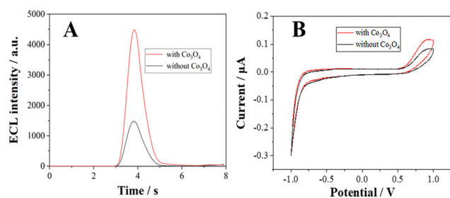
Fig. 1 (A) ECL profiles and (B) CV curves of the L12- \text{H}_2\text{O}_2 system at the ITO surface with and without \text{Co}_3\text{O}_4 . Working solution: 10 mM PBS containing 200 \mu\text{M} L12. Scan range: -1.0 to 1.0 V, scan rate: 0.1 V \text{s}^{-1} , PMT voltage: 600 V.
