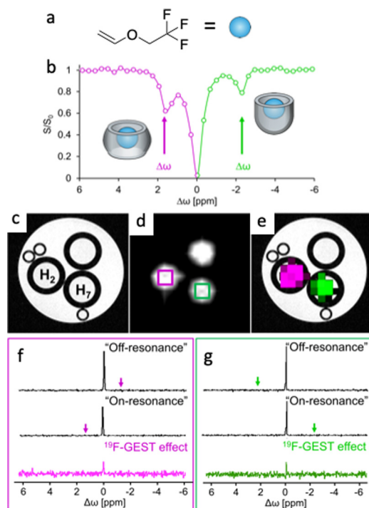
Fig. 9 Diamagnetic GEST: (a) the chemical structure of the fluorinated anesthetic fluoroene used as an inhalable ^{19}\text{F} -guest. (b) ^{19}\text{F} -GEST z-spectrum obtained from an aqueous solution containing a mixture of cucurbit[7]uril (H2) and dimeric octa acid (H7). The sample contained 5 mM fluoroene and 10 \mu\text{M} of each host. (c) ^1\text{H} -MRI, (d) ^{19}\text{F} -MRI, and (e) ^{19}\text{F} -GEST map of a three-tube phantom containing 5 mM fluoroene and 5 \mu\text{M} of either cucurbit[7]uril (H2) or octa acid (H7). A tube with 5 mM fluoroene only was used as a control. (f and g) Localized ^{19}\text{F} -GEST spectroscopy data of two voxels acquired from the tubes containing (f) H2:fluoroene (magenta) or (g) H7:fluoroene (green). The ^{19}\text{F} -GEST spectra represent the subtraction of the ^{19}\text{F} -NMR spectra obtained when the saturation pulse was applied "on-resonance" from the ^{19}\text{F} -NMR spectra obtained when the saturation pulse was applied "off-resonance." Data were acquired with a 9.4 T MRI scanner with B_1 = 2.5 \mu\text{T}/2 \text{ s} . For fluoroene@H2, "on-resonance" was \Delta\omega = +1.6 \text{ ppm} and "off-resonance" was \Delta\omega = -1.6 \text{ ppm} . For fluoroene@H7, "on-resonance" was \Delta\omega = -2.2 \text{ ppm} and "off-resonance" was \Delta\omega = +2.2 \text{ ppm} . Modified with permission from ref. 83.
