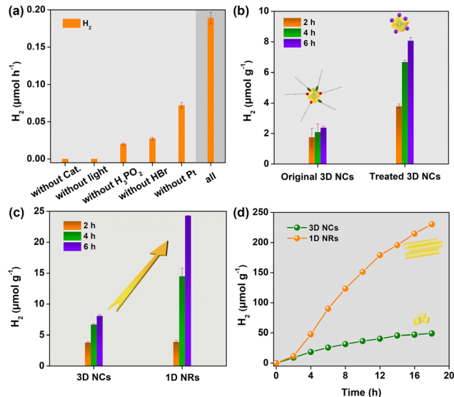
Fig. 2 (a) Control experiments of solar \text{H}_2 evolution in 2.0 h of irradiation over 3D NCs after ligand exchange ( \lambda \geq 400 nm). (b) Comparison of solar \text{H}_2 evolution between 3D NCs before and after ligand exchange under identical conditions. (c) Solar \text{H}_2 evolution with 3D NCs and 1D NRs capped with \text{BF}_4^- . (d) Solar \text{H}_2 production under optimal conditions with long irradiation time. Error bars represent mean \pm standard deviation (s.d.) of at least three independent experiments.
