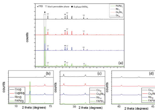
Fig. 1 X-ray diffraction patterns of the perovskite films (a) at full range and (bottom) with a focus at 10–15° (b), 28–33° (c), and 42–46° (d). The “ \nabla ” denotes the perovskite peaks and “ \bullet ” denotes the fluorine-doped tin oxide (FTO) peaks.
