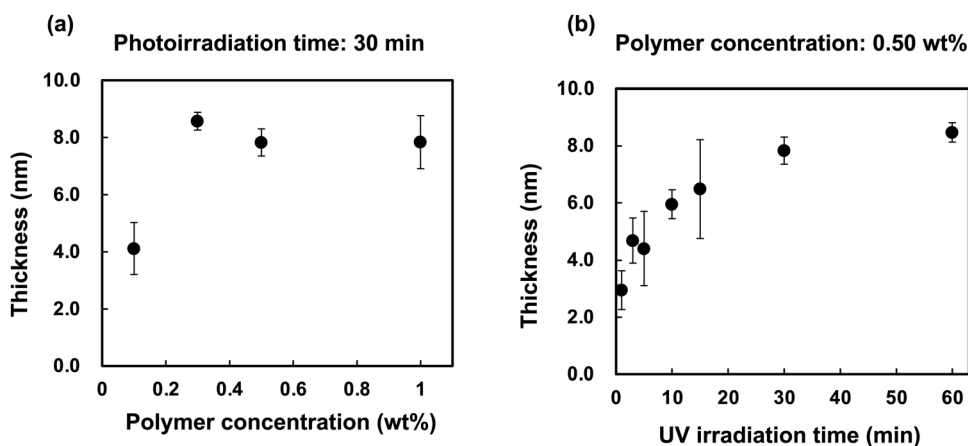
Fig. 3 (a) Relationship between the r-PMB layer thickness and polymer concentration. (b) Relationship between the thickness of the r-PMB layer and photoirradiation time.
