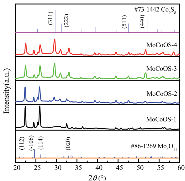
Fig. 2 XRD diffraction patterns of MoCoOS, the Mo 4 O 11 standard of PDF 86-1269, and the Co 9 S 8 standard of PDF 73-1442.
