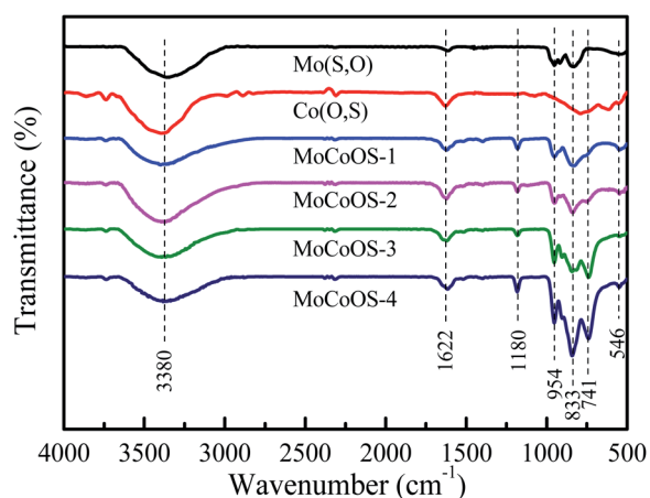
Fig. 3 FTIR spectra of Mo(S,O), Co(O,S), and MoCoOS prepared with different amounts of CoCl 2 ·6H 2 O.
