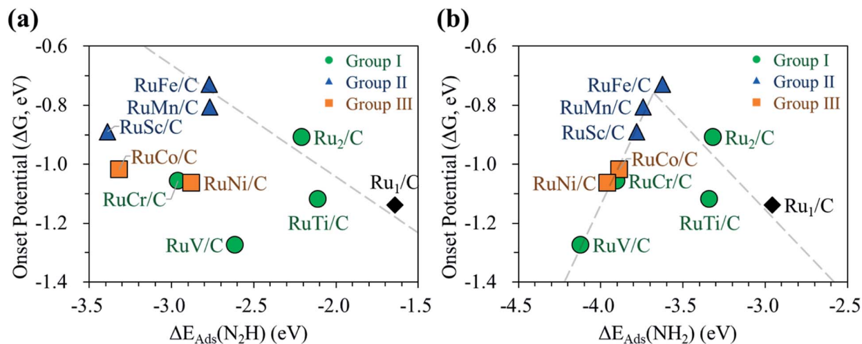
Fig. 7 Relationship between the onset potential of the \text{N}_2\text{RR} and the adsorption energies of (a) \text{N}_2\text{H} and (b) \text{NH}_2 . In (b), the PLS of the catalysts located on the left side of the peak position is (5) \text{NH}_2^* + (\text{H}^+ + \text{e}^-) \rightarrow \text{NH}_3(\text{g}) , while for the right-side case, the PLS is (6) \text{N}_2^* + (\text{H}^+ + \text{e}^-) \rightarrow \text{N}_2\text{H}^* .
