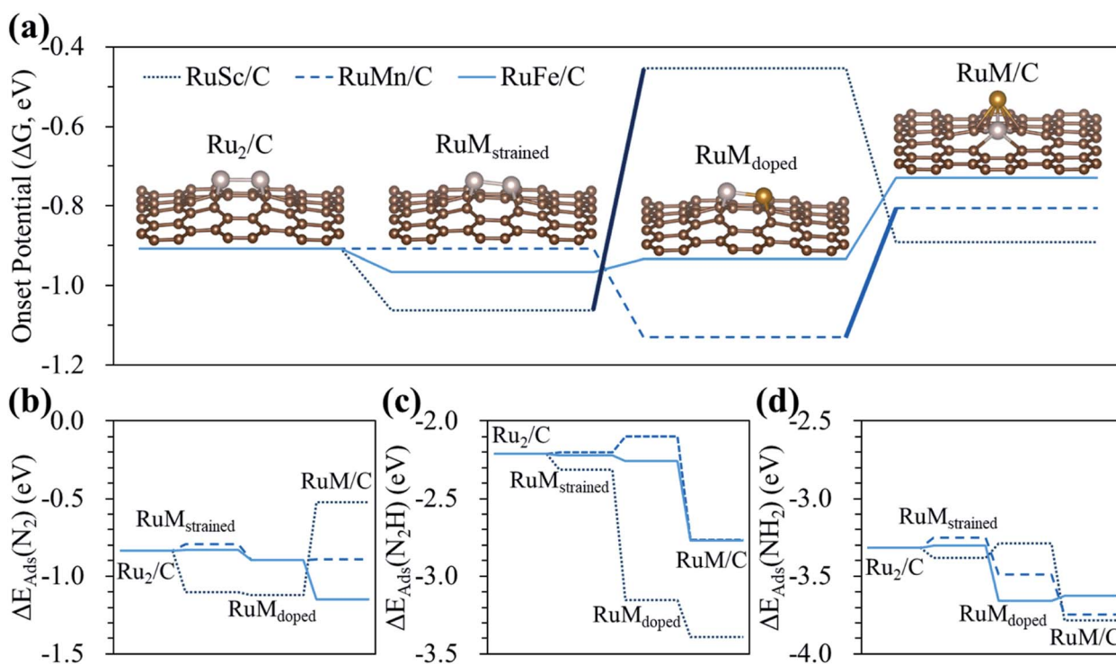
Fig. 8 Contribution of strain, dopant and configurational effects to the (a) onset potential, and adsorption energy of (b) \text{N}_2 , (c) \text{N}_2\text{H} , and (d) \text{NH}_2 of the \text{N}_2\text{RR} on the hetero- \text{RuM} DACs. In (a), the bold solid lines indicate the change in the limiting step from [\text{N}_2^* + (\text{H}^+ + \text{e}^-) \rightarrow \text{N}_2\text{H}^*] to [\text{NH}_2^* + (\text{H}^+ + \text{e}^-) \rightarrow \text{NH}_3(\text{g})] .
