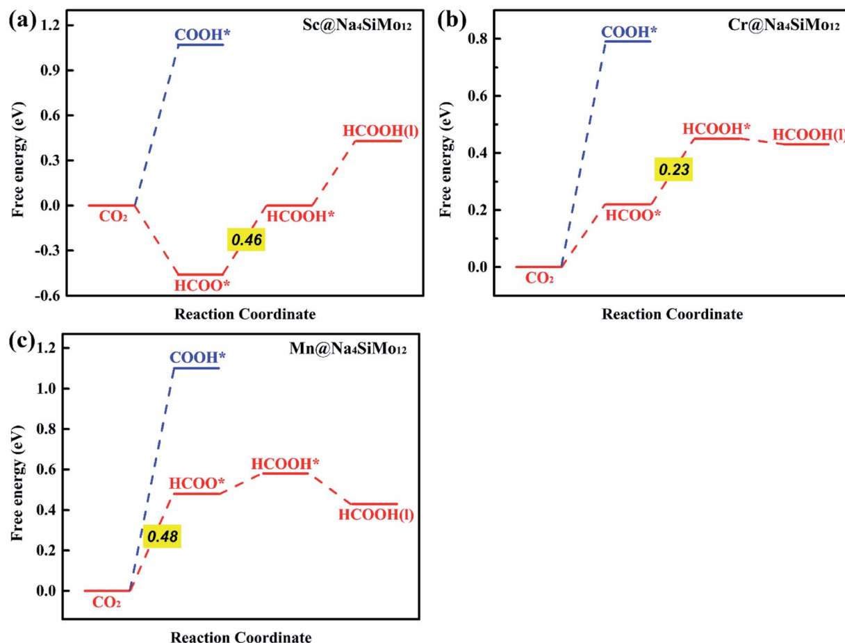
Fig. 6 Calculated free energy diagrams for the electrochemical \text{CO}_2 RR on (a) \text{Sc}@\text{Na}_4\text{SiMo}_{12} , (b) \text{Cr}@\text{Na}_4\text{SiMo}_{12} and (c) \text{Mn}@\text{Na}_4\text{SiMo}_{12} .
