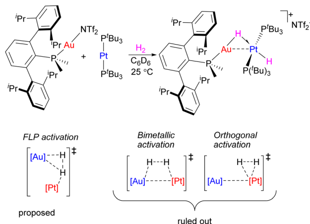
Scheme 11 H 2 activation by Pt 0 /Au I system and possible modes of cooperative H 2 activation.
