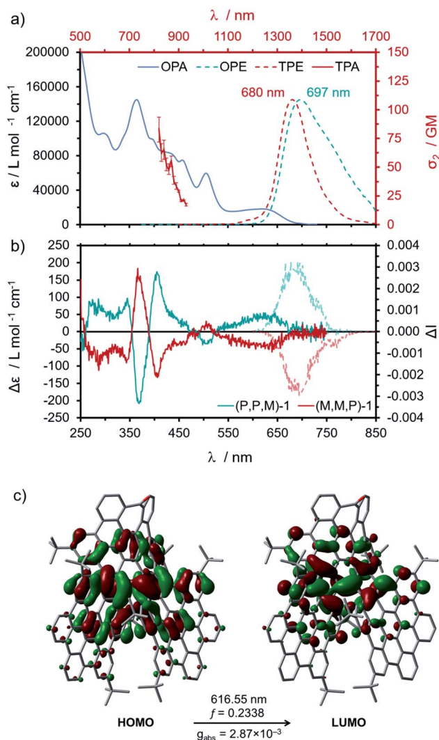
Fig. 3 (a) Experimental OPA (gray), OPE (turquoise, dashed), TPA (red) and TPE (red, dashed) spectra of (M,M,P,P,P,M)-1. Measured in CHCl 3 at ca. 1 \times 10^{-6} M, \lambda_{\text{exc}} = 370 nm for OPE, \lambda_{\text{exc}} = 900 nm for TPE; (b) experimental ECD spectra of (M,M,P)-1 (red) and (P,P,M)-1 (turquoise) measured in CHCl 3 at ca. 1 \times 10^{-6} M, and experimental CPL spectra ( \lambda_{\text{exc}} = 370 nm) of (M,M,P)-1 (pale red, dashed) and (P,P,M)-1 (pale turquoise, dashed) measured in CHCl 3 at ca. 1 \times 10^{-6} M; (c) HOMO and LUMO orbitals, and information of the TD-DFT calculated (CAM-B3LYP/6-31G(d,p)) lowest energy transition. The OPE spectrum is cropped at long wavelengths due to the use of a short path filter to block the multiphoton laser at the entrance of the photodetector.
