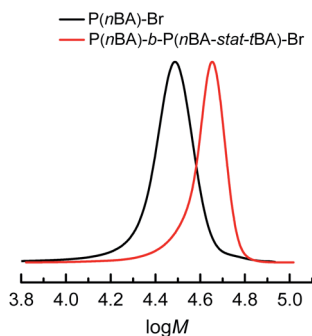
Fig. 5 Molecular weight distribution of P(nBA) 288 -Br macroinitiator ( M_n = 37.0 kDa and \bar{D} = 1.11 , conv. BA = 83%) and P(nBA) 288 -b-P(nBA 40 -stat-tBA 56 )-Br copolymer ( M_n = 50.6 kDa and \bar{D} = 1.06 , conv. tBA = 25%, conv. BA = 94%) produced by PGE eATRP of n BA and n BA + tBA at T = 45^\circ\text{C} in DMF + 0.1 M \text{Et}_4\text{NBF}_4 . tBA was added after 1 h of n BA polymerization under the following conditions: n\text{BA}/\text{EBiB}/\text{Cu}(\text{OTf})_2/\text{Me}_6\text{TREN}/\text{Et}_4\text{NBr} = 349/1/0.1/0.3/0.1 , C_{n\text{BA}} = 3.49 M.
