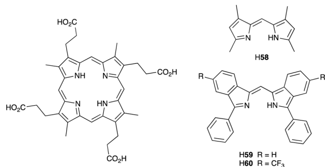
Scheme 22 Structures of the porphyrin H 2 CPI, and three Hdipyrin ligands.
