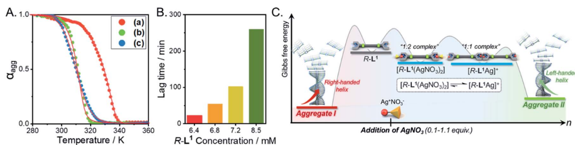
Fig. 8 (A) Degree of aggregation at 326 nm as a function of temperature with the heating curve fitted to the equilibrium (EQ) model regime based on the nucleation–elongation model; 58–60 (a) aggregate I, (b) aggregate II, and (c) aggregate III. (B) Representation of the lag time concentration in the presence of 0.6 equiv. AgNO_3 in a mixture of DMSO and H_2O (1 : 1 v/v). (C) Energy landscapes of the two competing pathways of R-L^1 in the presence of AgNO_3 : elongation Gibbs free energies were experimentally determined by using the cooperative supra-molecular polymerization model.
