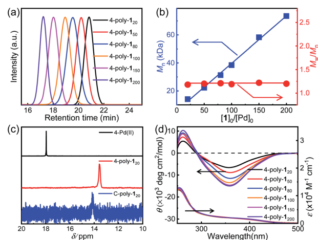
Fig. 1 (a) SEC curves of 4-poly- 1 n polymers with different M_n s. (b) Plot of M_n and M_w/M_n values of 4-poly- 1 n polymers as a function of the 1 -to-Pd(II) ratio. (c) 31 P NMR spectra of 4-Pd(II) , 4-poly- 1 20 , and C-poly- 1 20 . (d) CD and UV-visible spectra of 4-poly- 1 n polymers measured in THF at 20^\circ\text{C} .
