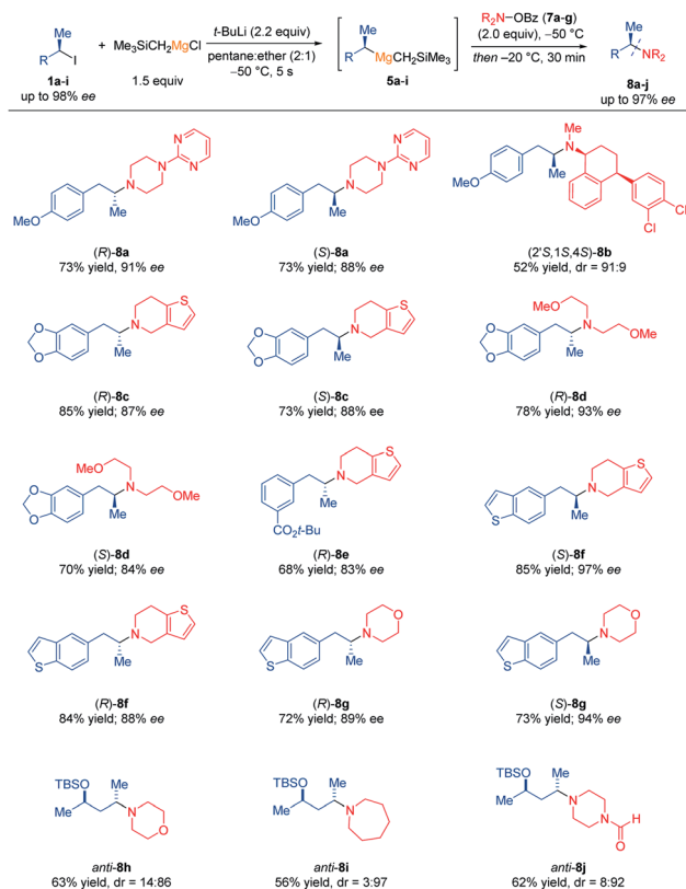
Scheme 3 Scope of prepared enantiomerically and diastereomerically enriched \alpha -chiral tertiary amines. Enantiomerically and diastereomerically enriched tertiary amines 8a–j obtained by electrophilic amination of secondary alkylmagnesium reagents 5a–i with O -benzoyl hydroxylamines ( 7a–g ). The enantiomeric excess (% ee) was determined by chiral HPLC-analysis. The diastereomeric ratio (dr; syn / anti ratio) was determined by ^1\text{H} -NMR spectroscopy and GC-analysis.
